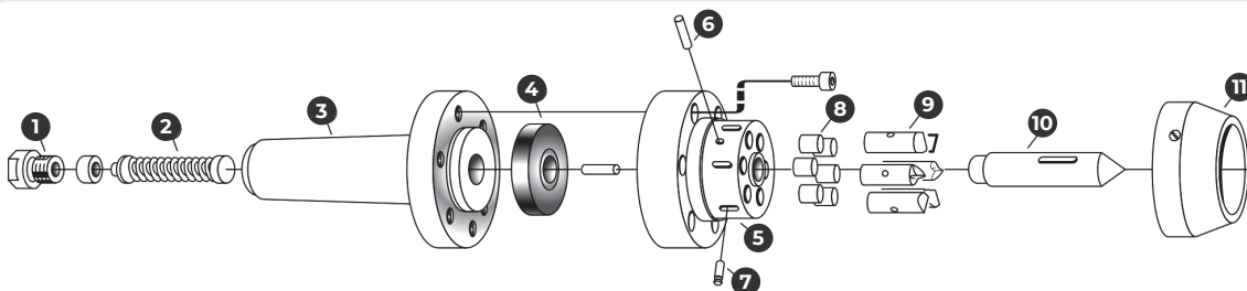
1 End cover 2 Spring rod 3 Shank 4 SP urethane 5 Head 6 Pin At Point 7 Pin At Pin 8 Roller 9 Drive pin 10 Center Point 11 Cover
