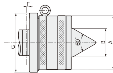
Available Draw-off Nut Type HSN-TYPE
